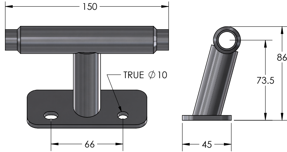
ESU26y261 AXLE SIZE 15MM X 150MM
