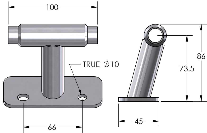
ESU26y211 AXLE SIZE 15MM X 100MM
