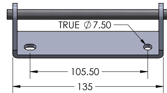
ESU:y246 AXLE SIZE 9MM X 135MM
