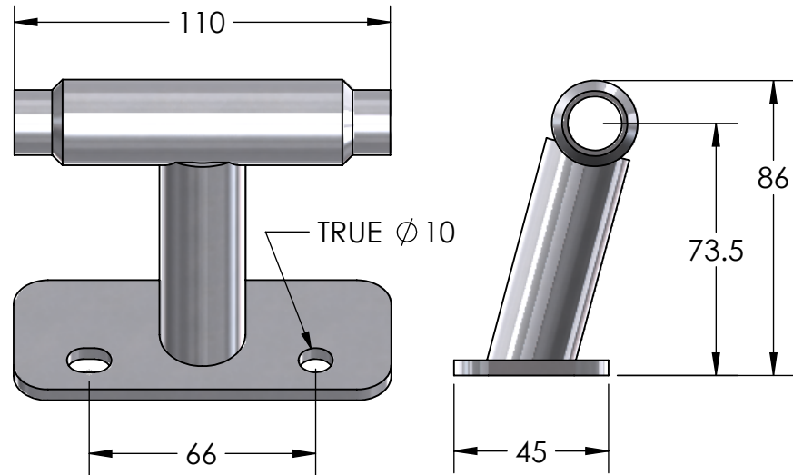
ESU26y221 AXLE SIZE 15MM X 110MM
