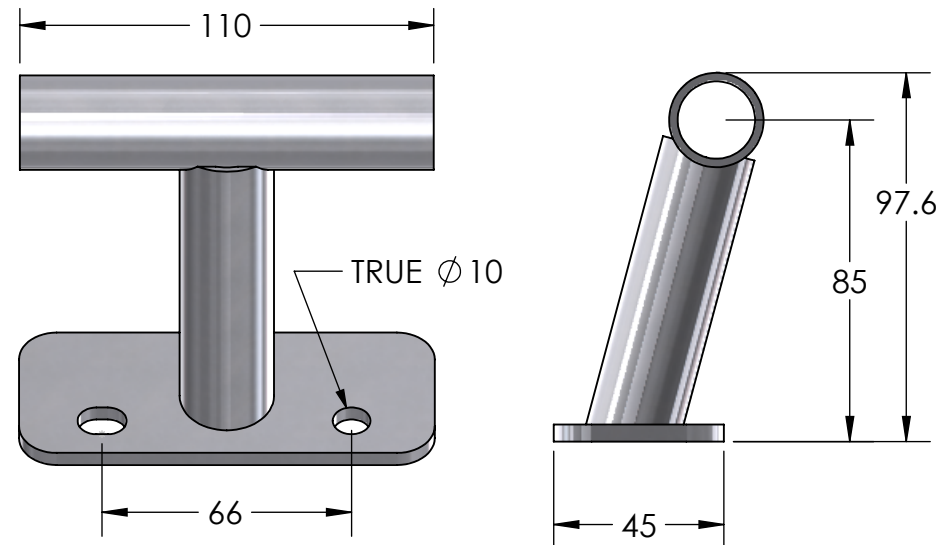
ESU31y221 AXLE SIZE 20MM X 110MM
