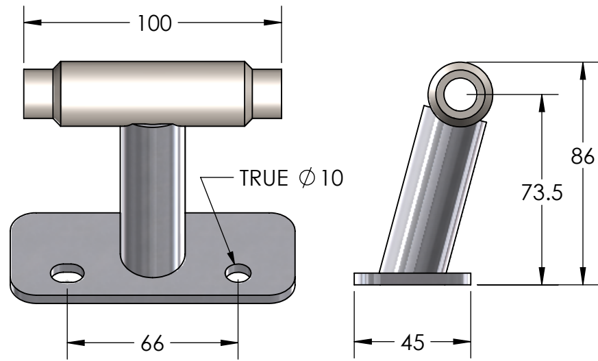
ESU26y211 AXLE SIZE 15MM X 100MM
