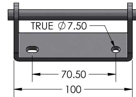
ESU:y211 AXLE SIZE 9MM X 100MM
